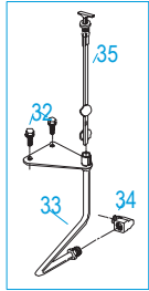
Dipstick components
